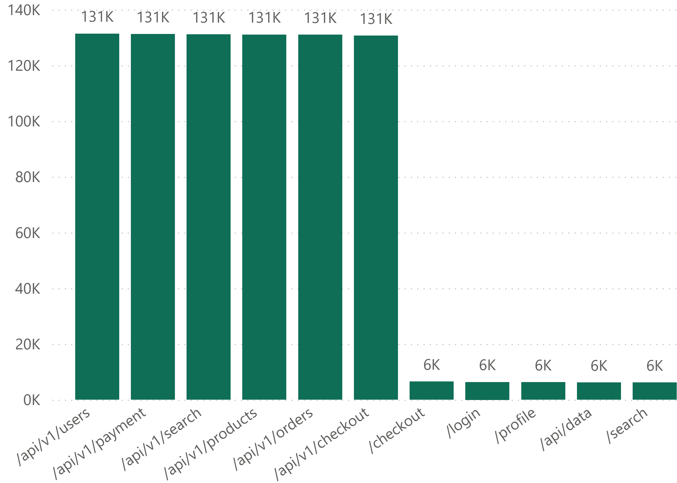
Total requests by endpoint
