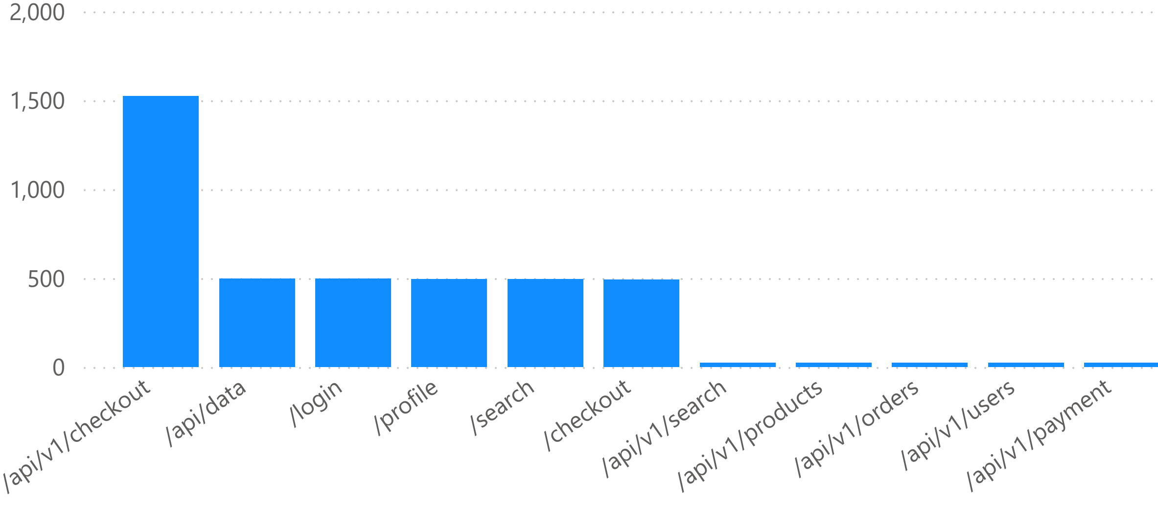
Avg Execution Time by endpoint
