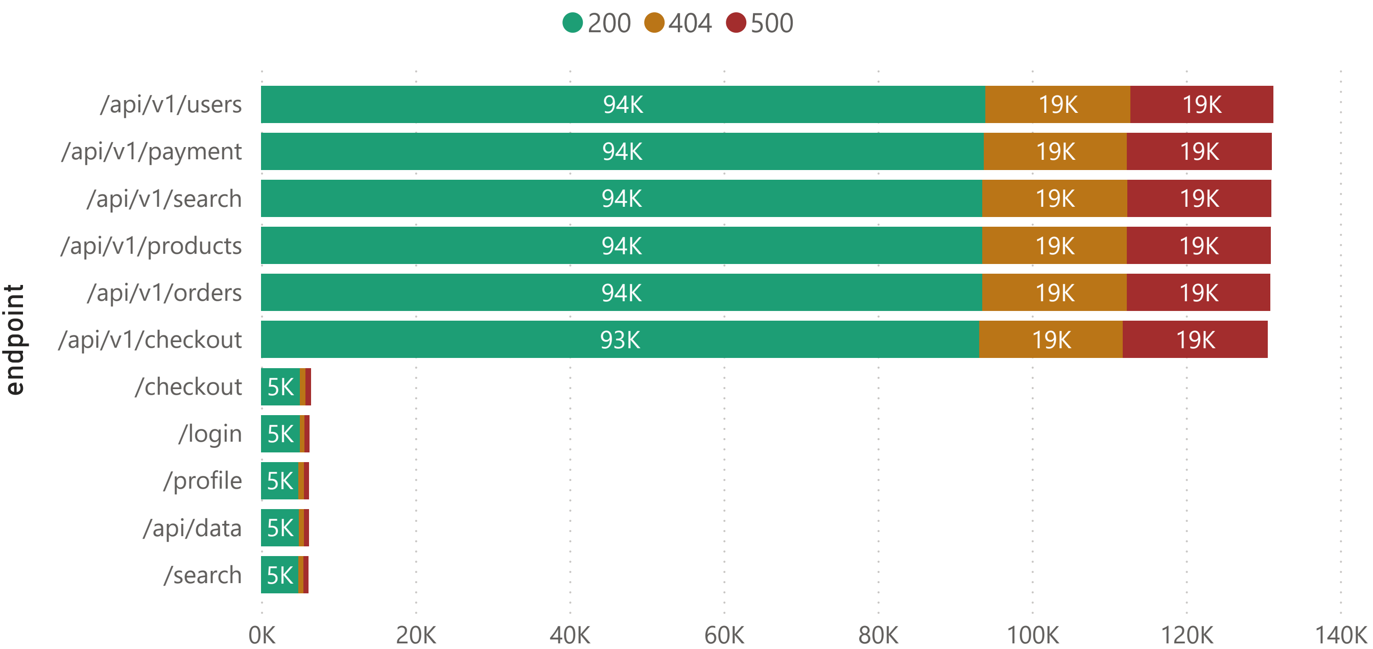
Total Requests by endpoint and status
